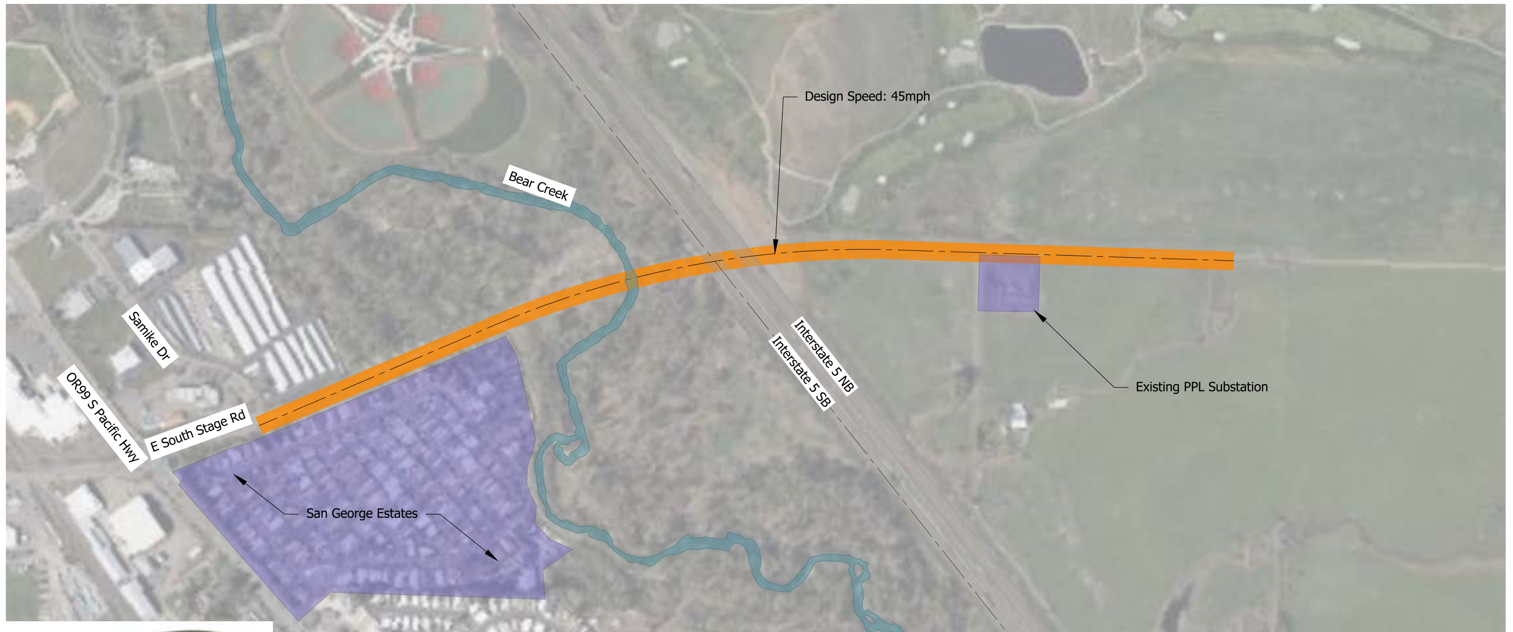
Figure O-1 Overpass Alternative 1
